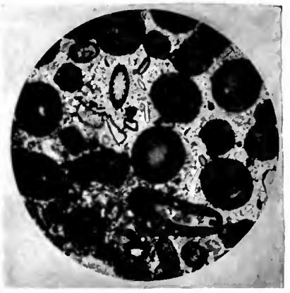
FIG. 3.—CRINOIDAL LIMESTONE (CARBONIFEROUS), CLIFTON, NEAR BATH, ENGLAND ( \times 10 ).
