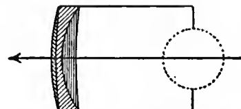
FIG. 16.—Rapid Landscape Lens. Long Focus.
