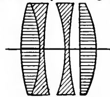
FIG. 51.—Zeiss's "Tessar."
