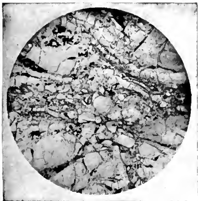
FIG. 4.—PERLITIC OBSIDIAN, TOKAI, HUNGARY ( \times 15 ).
