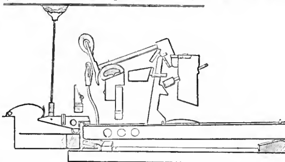
FIG. 24.—Broadwood's Grand Piano Action, 1884. English direct mechanism.
