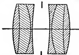
FIG. 36.—Steinheil's "Orthostigmat."
