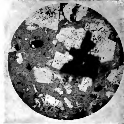
FIG. 3.—TRACHYTE, PERLENHARDT, GERMANY ( \times 10 ).
