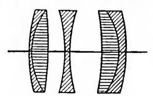
FIG. 52.—Voigtlander's "Heliar."
