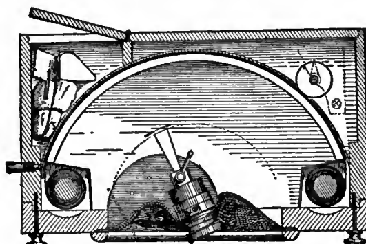
FIG. 11.—Section of "Al-Vista" Panoramic Camera.
