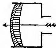
FIG. 15.—Grubb's "Aplanatic" Lens.
