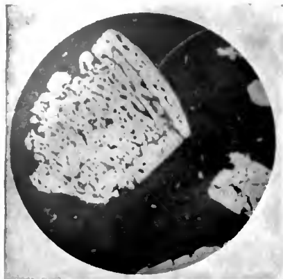
FIG. 1.—PORPHYRITIC PITCHSTONE, SCUR OF EIGG, SCOTLAND ( \times 10 ).
