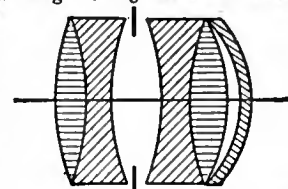
FIG. 42.—Stigmatic Lens. Series II.
