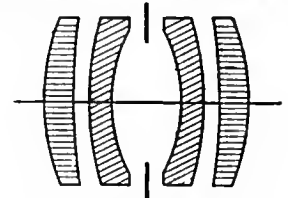
FIG. 50.—Ross's "Homocentric."
