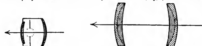
FIG. 27.—Wide-Angle Rectilinear Lens.
