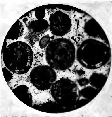
FIG. 5.—OOLITIC CHERT (CAMBRIAN), SUTHERLANDSHIRE, SCOTLAND ( \times 15 ).
