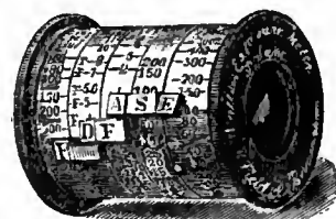
FIG. 69.—Watkins's "Standard" Meter.
