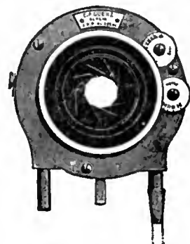
FIG. 67.—Goerz's "Sector" Shutter.
