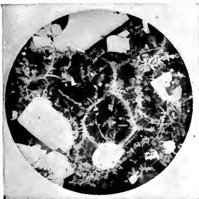
FIG. 7.—SPHERULITIC RHYOLITE, HLINIK, HUNGARY ( \times 10 ).
