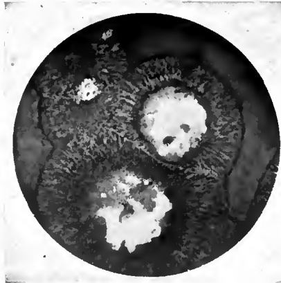
FIG. 8.—SPHERULITIC FELSITE, ARRAN, SCOTLAND ( \times 10 ).
