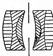
FIG. 35. Ross-Goerz "Dagor." Series III.
