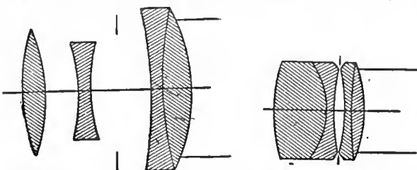
FIG. 21.—Portrait Aplanat. FIG. 22.—Group Aplanat. Form I. of 1874, but was superseded in 1881 by the "Portrait Aplanat," f/4 and free from astigmatism over an angle of 14^\circ .
