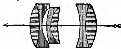
FIG. 41.—Stigmatic Portrait Lens. Series I.
