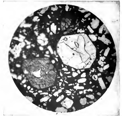
FIG. 3.—LEUCITE-BASANITE, VESUVIUS ( \times 8 ).
