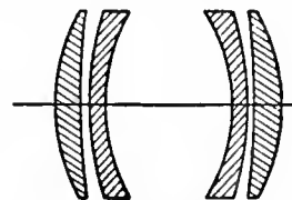
FIG. 49.—"Omnar," Series III.
