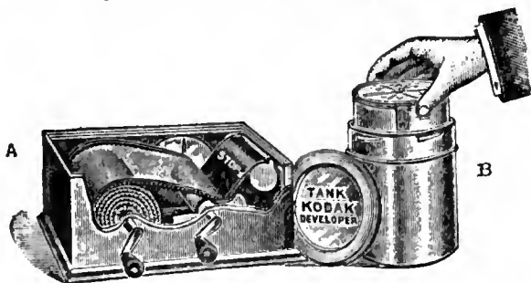
FIG. 74.—Kodak Developing Tank.
