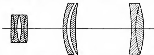
FIG. 57.—T. R. Dallmeyer's Compound Telephotographic Lens.
