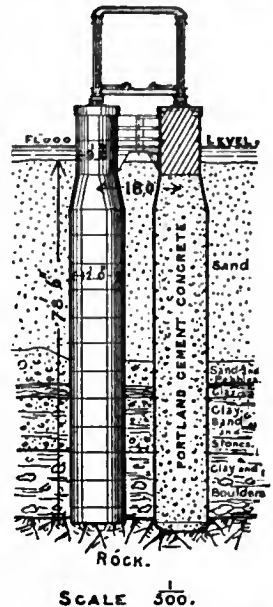
FIG. 2.—Cylindrical Piers for River Bridges.
