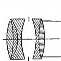
FIG. 23.—R. Steinheil's Improved Group Aplanat.
