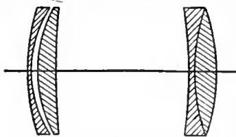
FIG. 20.—Dallmeyer's Patent Portrait Lens.
