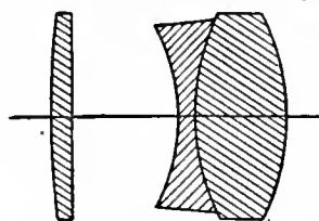
FIG. 48.—Aldis Lens. Series III.
